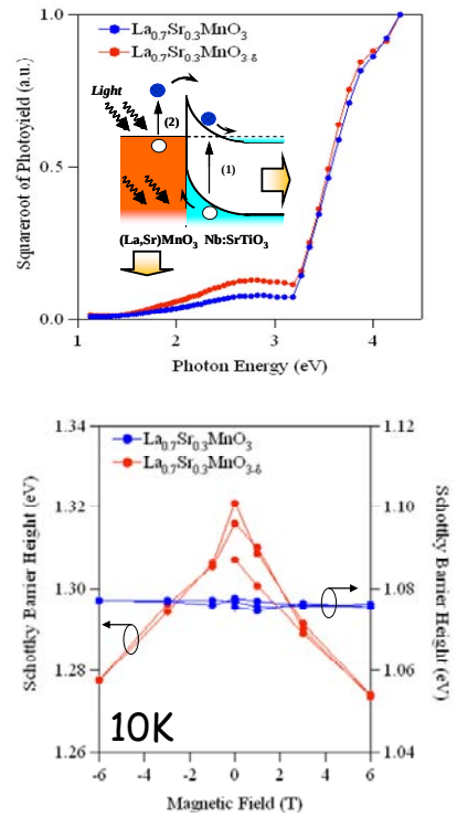
Fig. 2. The top panel shows the photocurrent yield as a function of photon energy. The two principle features observed are the \text{SrTiO}_3 bandgap and the Schottky barrier height. The bottom panel shows the evolution of the barrier height with applied magnetic field. Only the magnetically active \text{La}_{0.7}\text{Sr}_{0.3}\text{MnO}_{3-\delta} junction exhibits field dependence.
