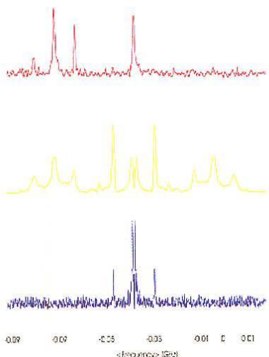
2 frequency Soft-ESEEM (top) vs. high-power and low-power ESEEM (middle and bottom, resp.) demonstrating the increased resolution.
