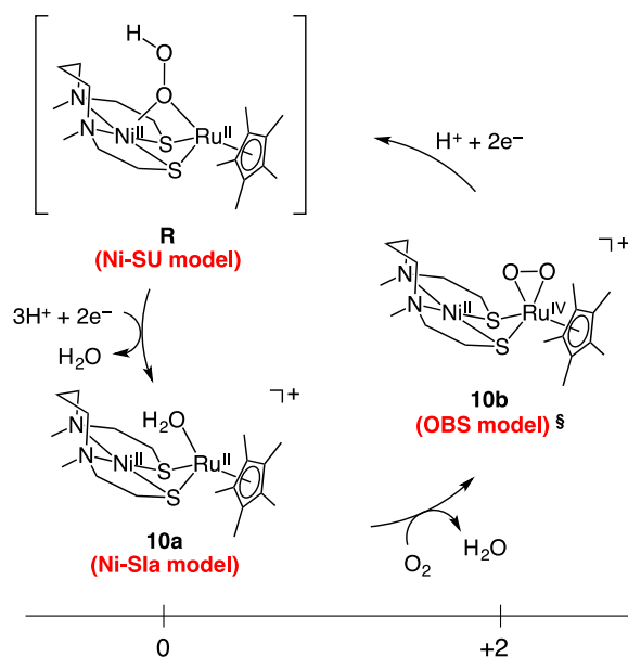
図27 カソードの反応メカニズム、§: a model complex for \text{O}_2 -bound species
